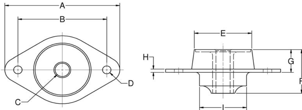
Figure 2 – Installation View (Shown Under No Load)
