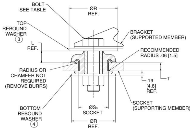
Figure 4 – Installation View (Shown Under No Load)
