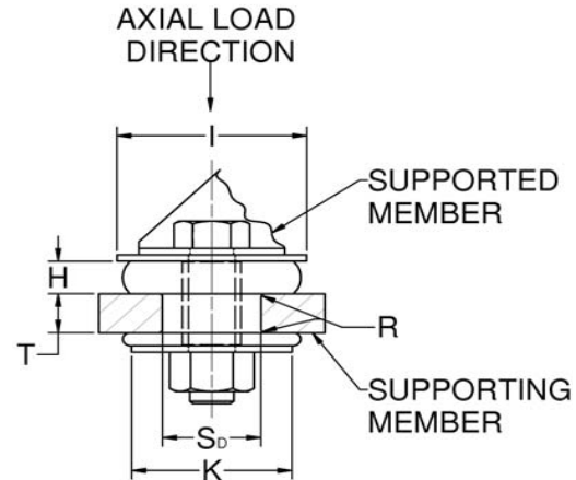
Figure 3 – Installation View (Shown Under No Load)
