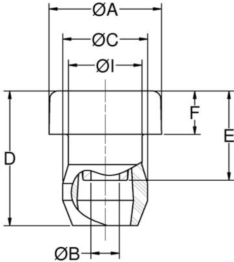
Figure 1 – Part Dimensions
