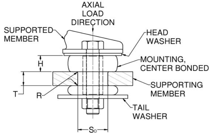
Figure 2 – Installation View (Shown Under No Load)
