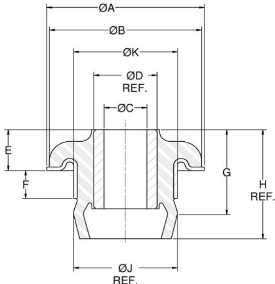
Figure 3 – Part Dimensions
