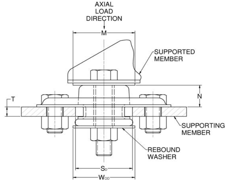
Figure 2 – Installation View (Shown Under No Load)
