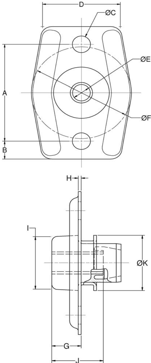
Figure 1 – Part Dimensions
