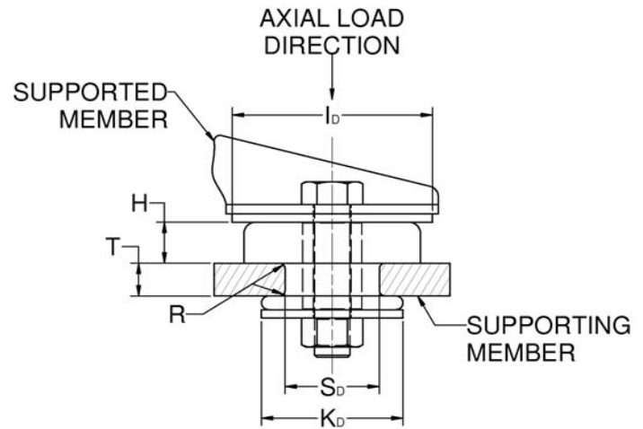
Figure 2 – Installation View
