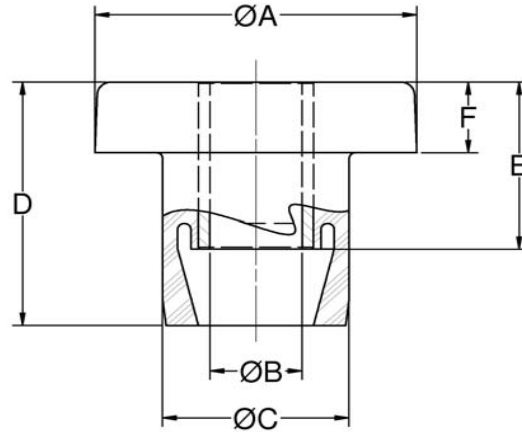
Figure 1 – Standard Series (Uninstalled)
