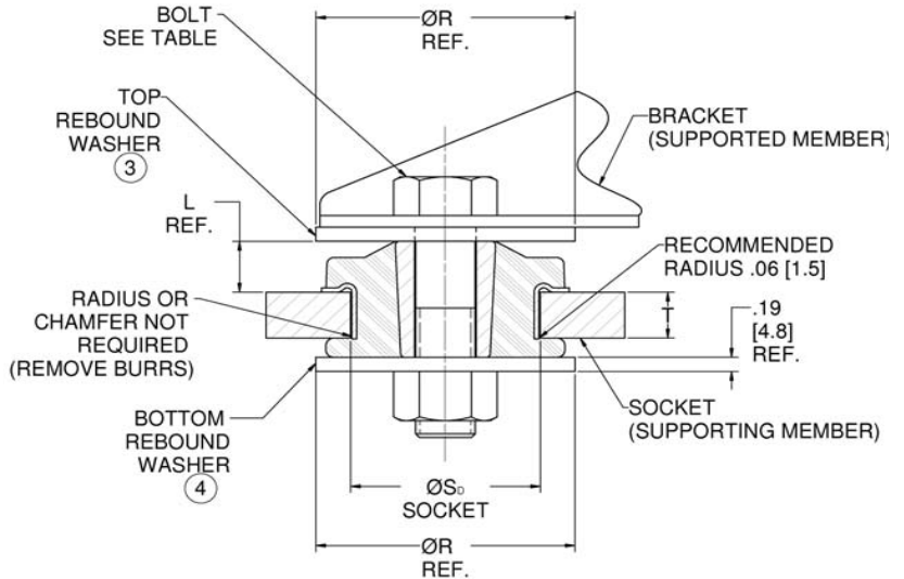
Figure 2 – Installation View (Shown Under No Load)
