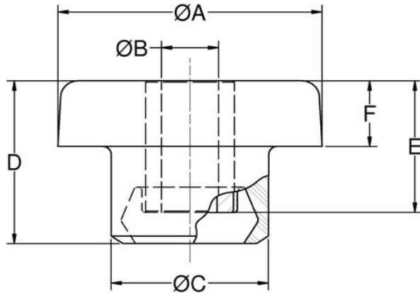
Figure 1 – Part Dimensions
