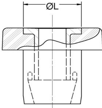
Figure 2 – High Bolt Torque Series (-1 Parts, Uninstalled, Flanged Inner Member)
