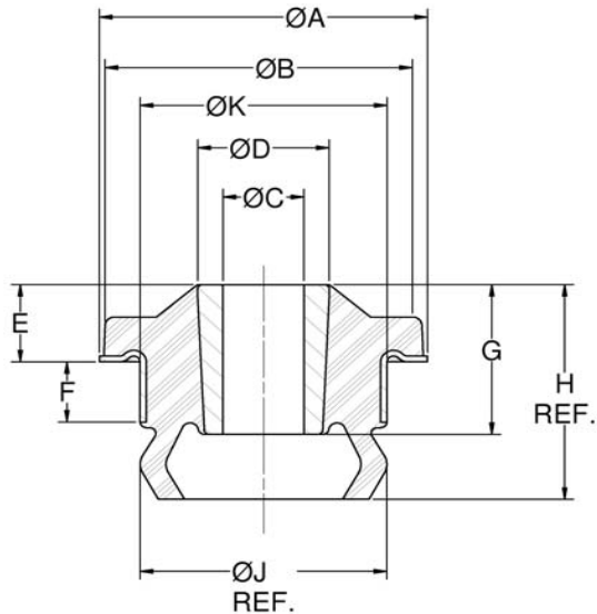
Figure 1 – Part Dimensions
