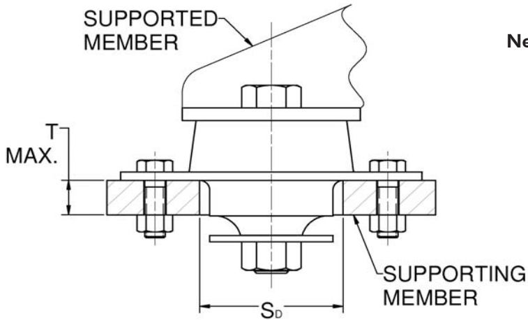
Figure 1 – Part Dimensions
